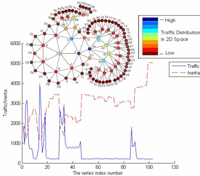
Figure 2: Traffic and inertia versus vertex number on a planar graph of valence 7; the graph has been made asymmetric so that the conjecture could be verified on cases where the centroid does not coincide with the obvious symmetry center. The centroid occurs at vertex #14. Also observe the heavy traffic at vertex #4, because it is the gateway between the top appendix and the right side of the network. Observe the “opposite phase” phenomenon between the inertia and the traffic, clearly seen for vertex #86.
