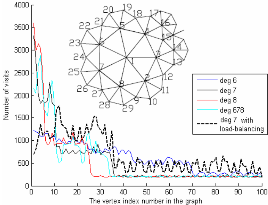
Figure 1: Top: Almost symmetric negatively curved network of valence 7. Bottom: Traffic function \tau versus vertex number; clearly, congestion at centroid increases as curvature becomes more negative. Also shown is the traffic function after curvature-based load balancing (see [19] for details).
