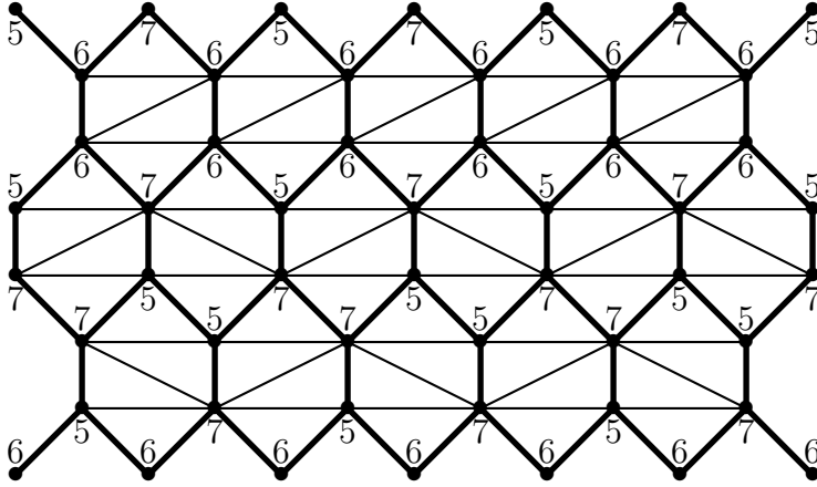
Figure 3: Planar triangulation with minimum degree 5 and low repetition.
