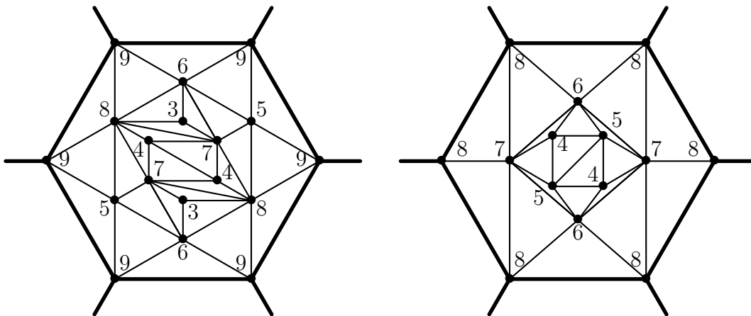
Figure 2: Tiles for planar triangulation with minimum degrees 3 and 4.
