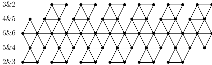
Figure 1: Maximal outerplanar graph with small repetition number.
