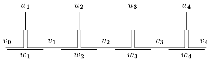
Fig. 3. Optimal proper subtree representation of G_4 .
