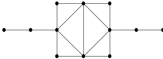
Fig. 2. A graph with a(G) > w(P'(G)) .
