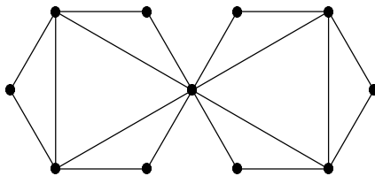
Fig. 1. A graph with leafage 4 but no asteroidal 4-set
