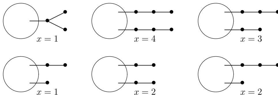
Figure 1: Possibilities for G in Theorem 1.5.
