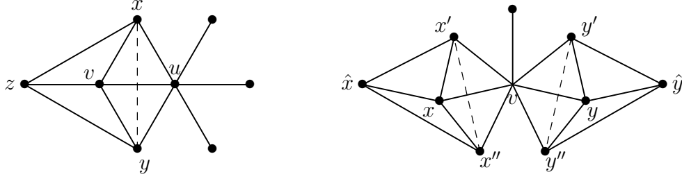
Figure 17: Cases 2 and 3 of Theorem 7.2
