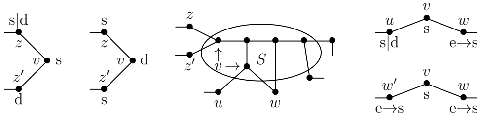
Figure 26: Induction for components of H in Theorem 7.18
