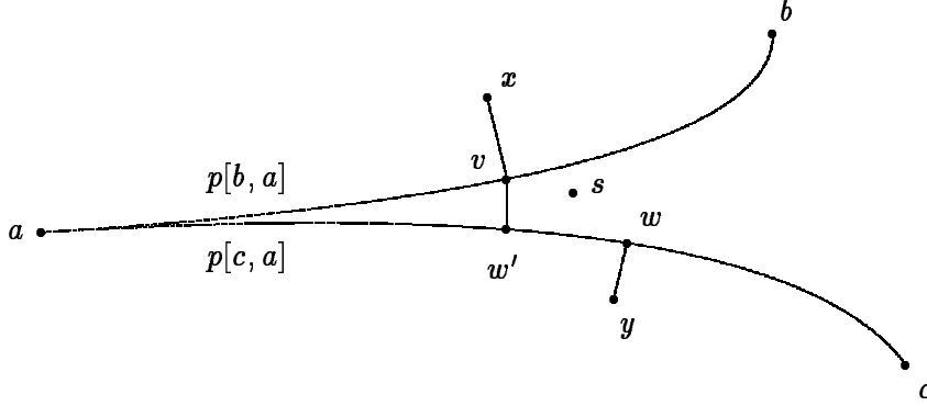
Figure 3: Proof of Proposition 7(6).
