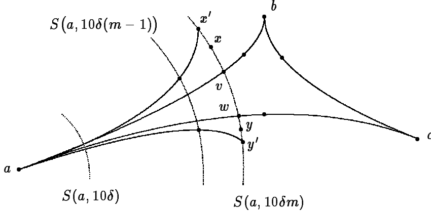
Figure 2: Proof of Proposition 3(5).
