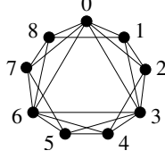
Figure 1: The graph H_9 .
