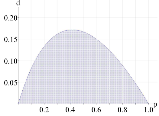
Figure 3: The graph of g_{K(1,2)}(p) .
