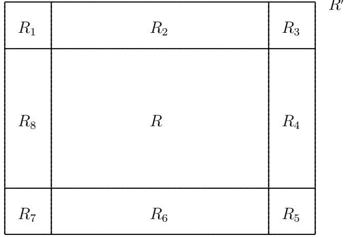
Figure 2: The rectangles R \subset R'
