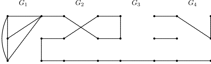
Figure 3: A graph G_{\mathcal{P}} , with S = [3] and m = 4 .
