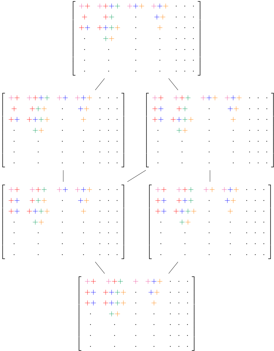
FIGURE 3. The subset of \text{Multi}(5361724) with support \mathcal{P} (cf. Example 3.7).
