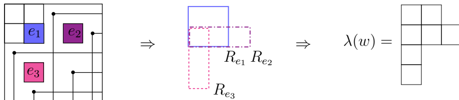
FIGURE 1. The diagram of w = 35142 (with color coded essential set \{e_1, e_2, e_3\} ), the overlay of R_{e_1}, R_{e_2}, R_{e_3} , and the shape \lambda(w) .
